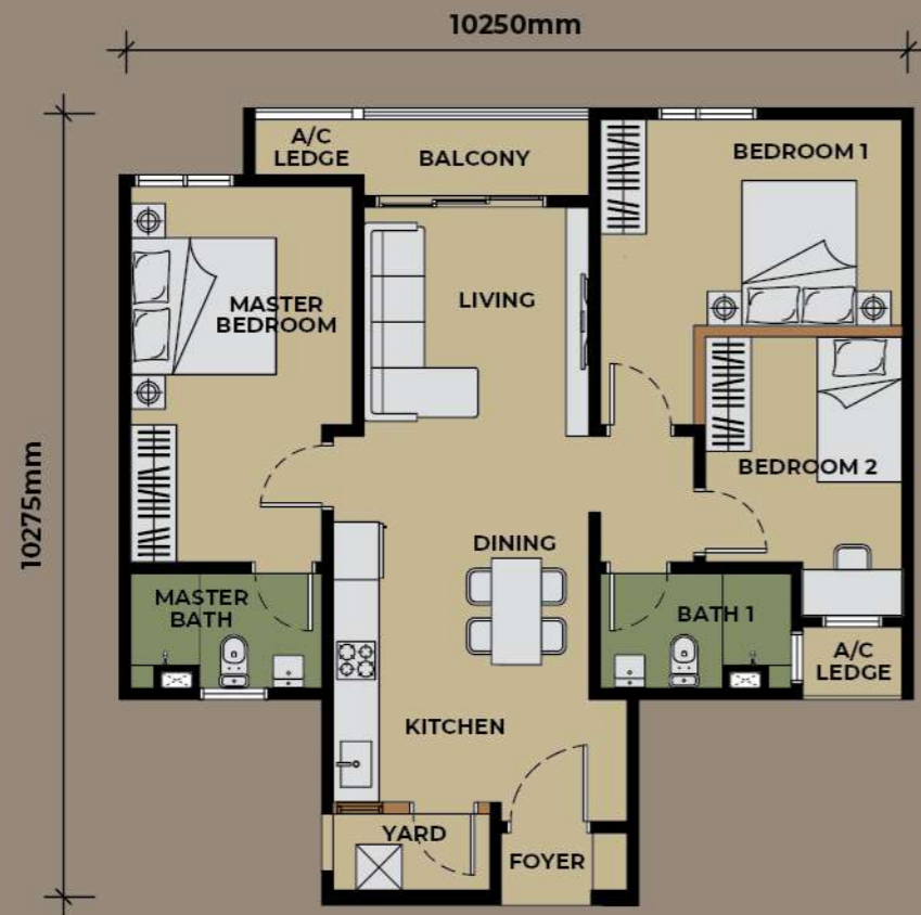
TYPE D1 (3R + 2B) 926 sq.ft. | 86 sm (Balcony)
